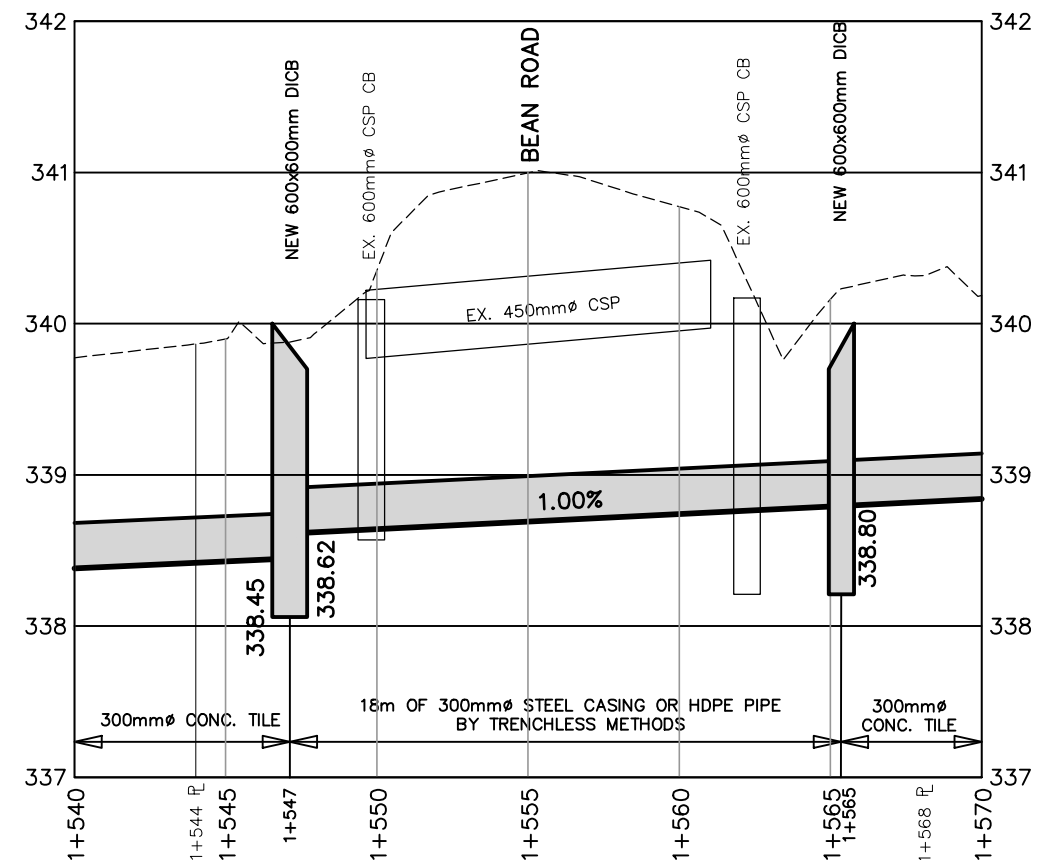
BEAN ROAD CROSSING - BRANCH 1
