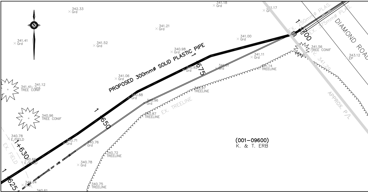
STA. 1+625 TO 1+698: DETAIL (ERB YARD)
