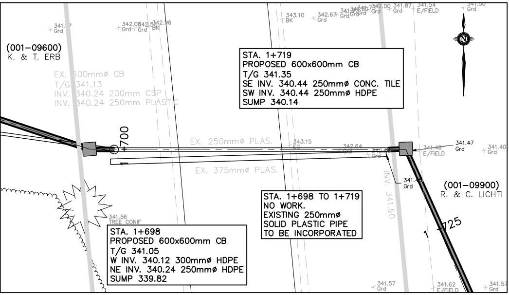
DIAMOND ROAD CROSSING DETAIL - BRANCH 1 (EXISTING)
